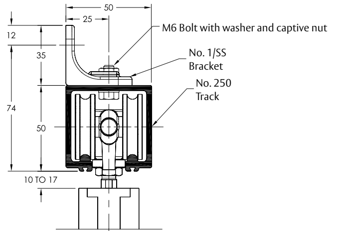
VIEW SHOWING ALTERNATIVE NO. 250 TRACK AND 1/SS BRACKET
