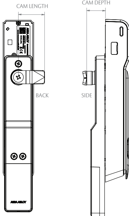
Diagram 2: Cam
