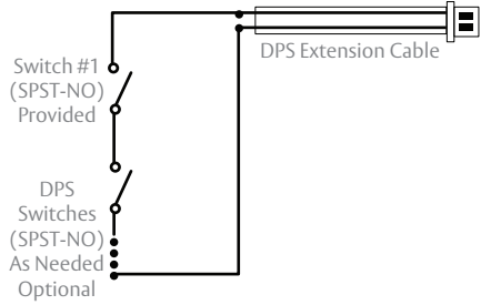
Diagram 8: DPS Cable
