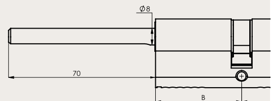
Optional: With 70 mm spindle replacing the thumbturn.
