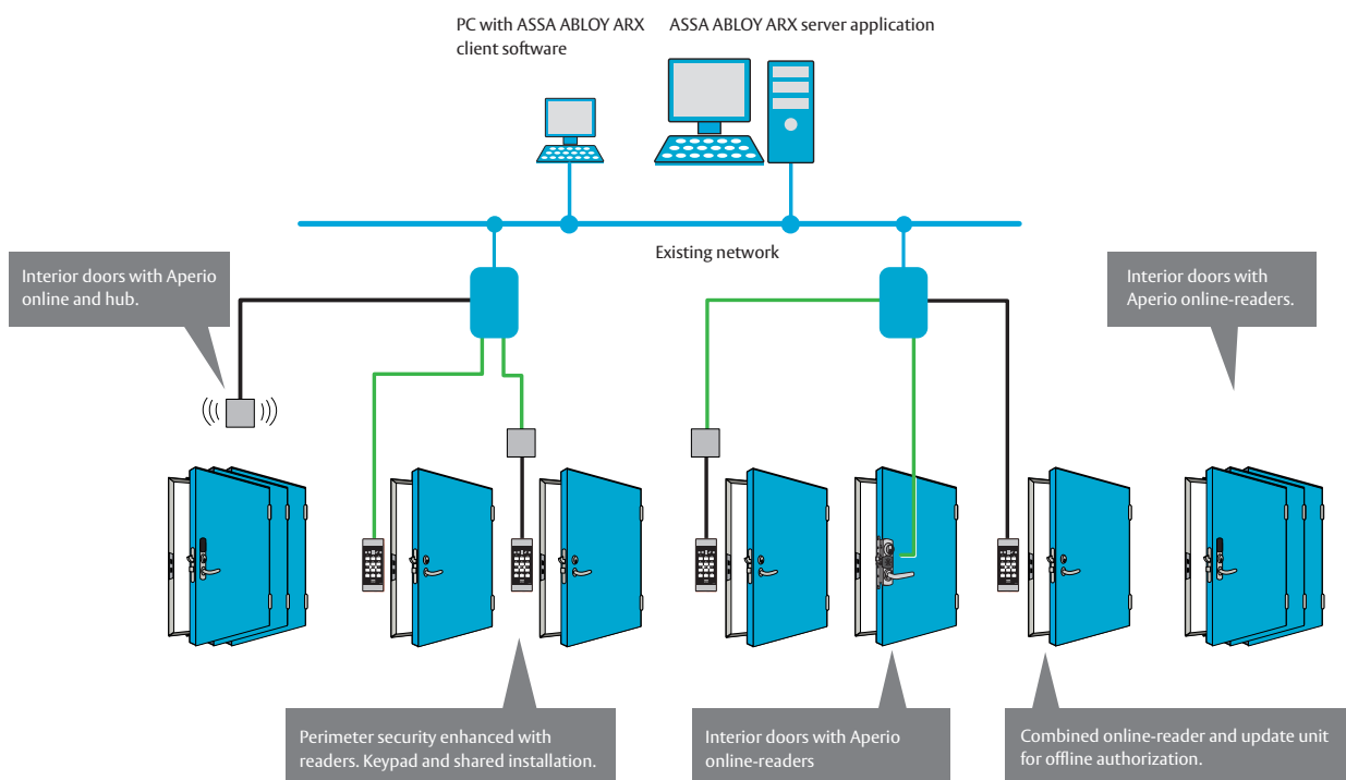
Functional diagram/example of system structure
